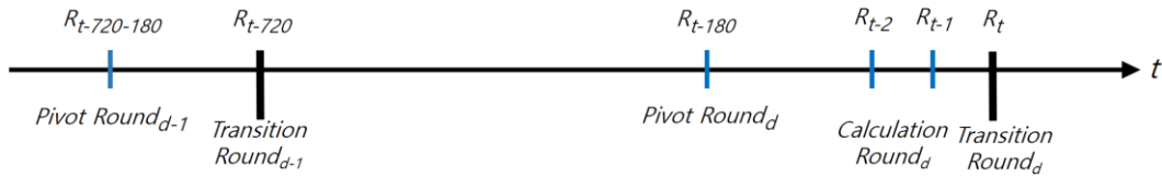
Figure 10: Epoch Pivot Round, Epoch Calculation Round, and Epoch Transition Round
