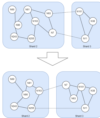
Figure 55: Shard Reconstruction through Node Migration
