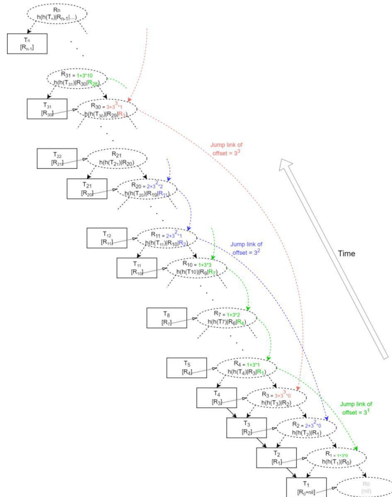
Figure 77: A Hierarchical SMT of base=3
