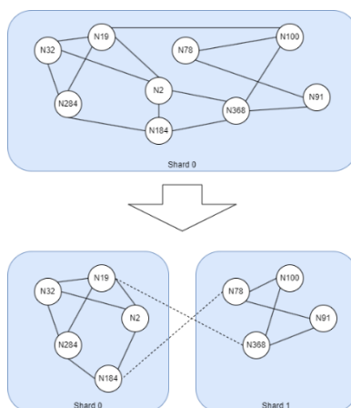
Figure 66: Increasing Shard Count through Shard Splitting
