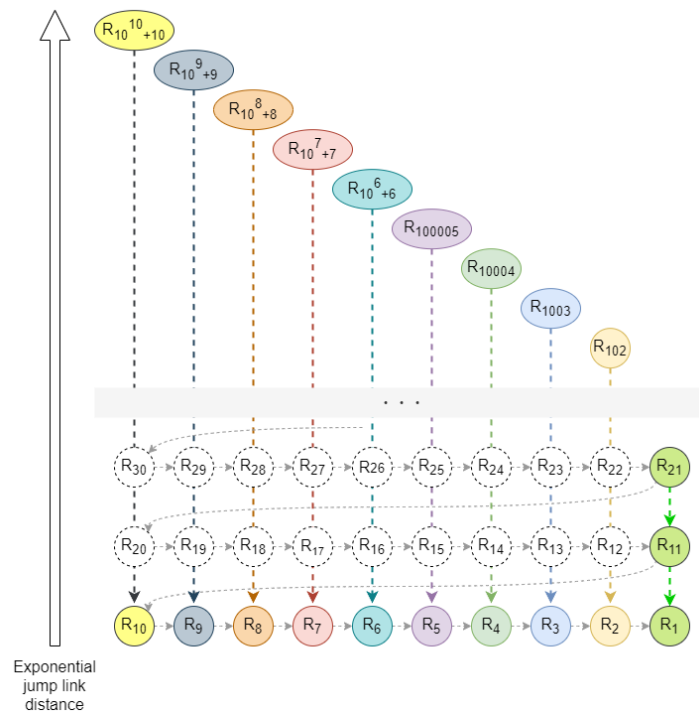
Figure 88: Hierarchical Skewed Merkle Tree and Jump Links exceeding exponential distances.
