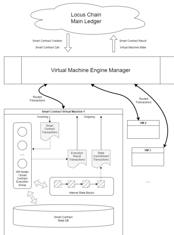
Figure 99: Locus Chain VME Structure
