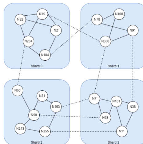
Figure 44: Locus Chain Node Sharding and P2P Communication Concept Diagram
